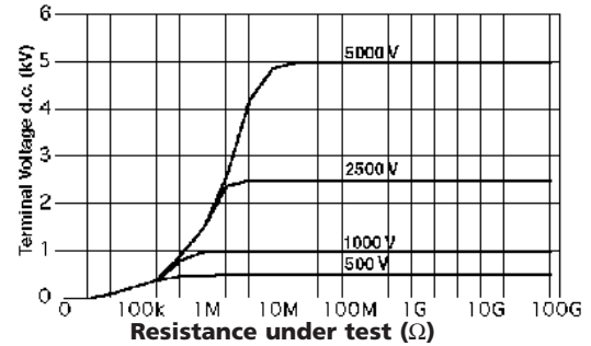
Typical Terminal Voltage Characteristics
