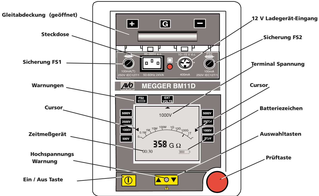
BM11D Frontplatten-Layout
