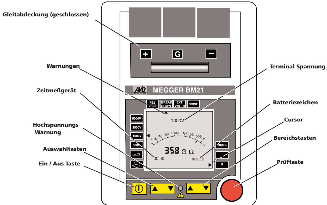
BM21 Frontplatten-Layout
