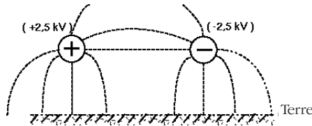
Figure 1. Essai flottant
